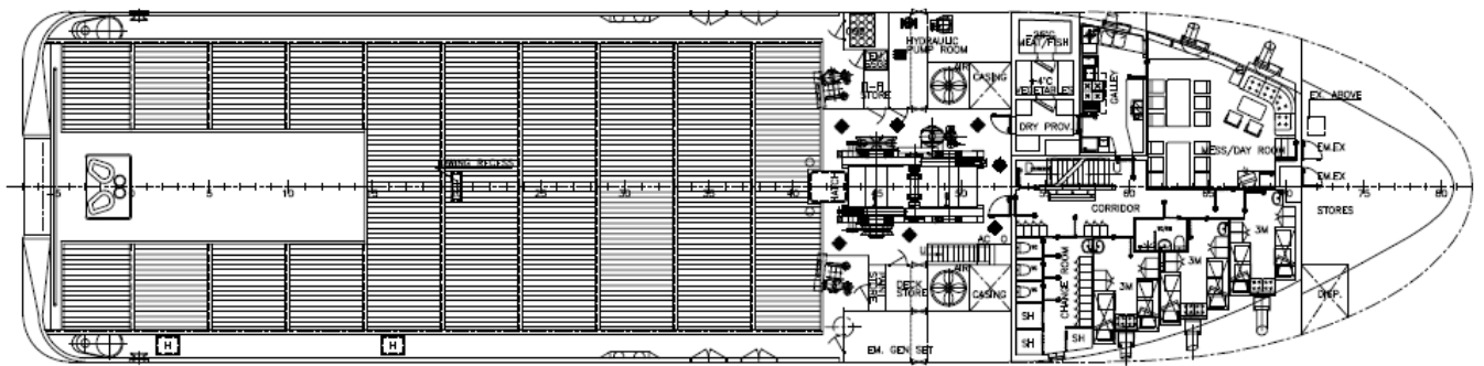
MAIN DECK
