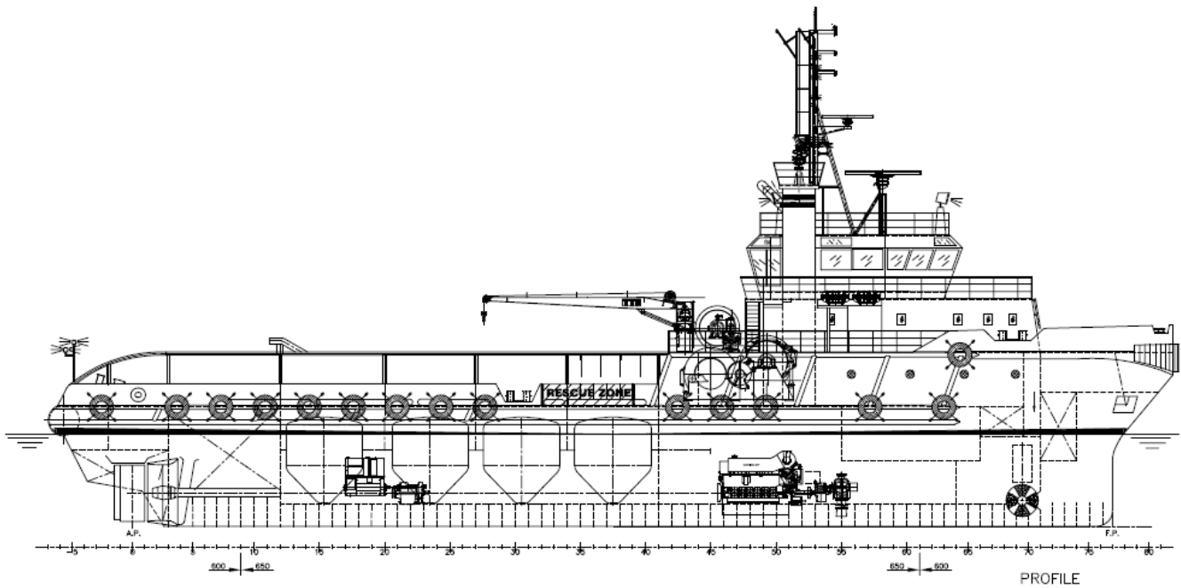
PROFILE
