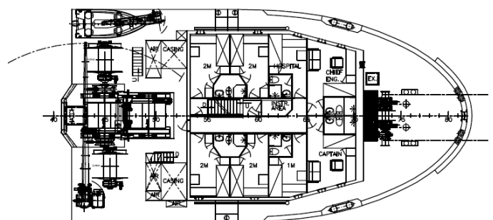
FORECASTLE DECK
